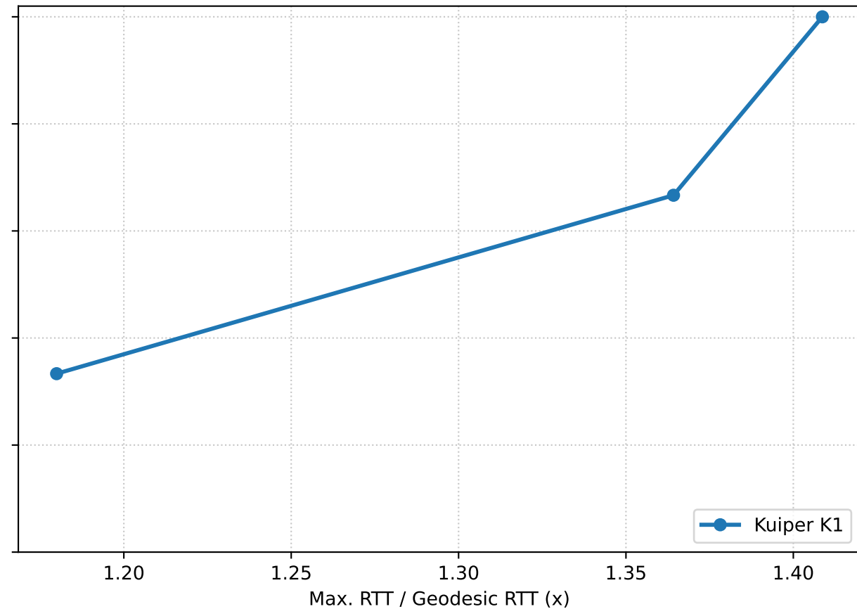
Multilayer
