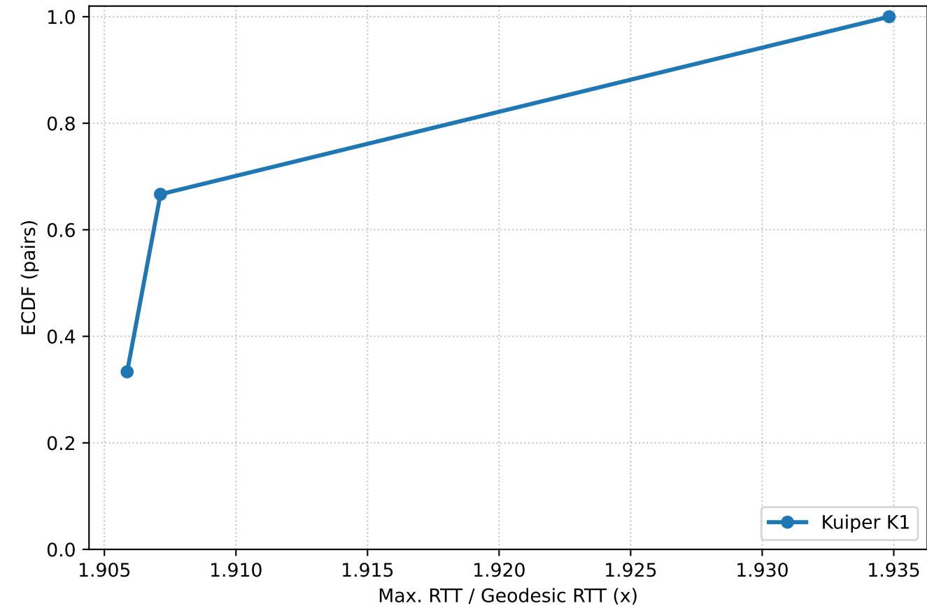
LEO-only
